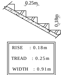
STAIRS DETAILS
