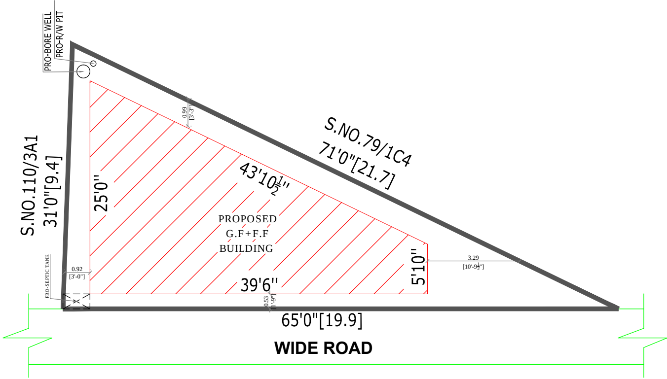
SITE PLAN SCALE: 1 INCH = 8 FEET
