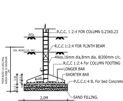
FOUNDATION DETAIL
