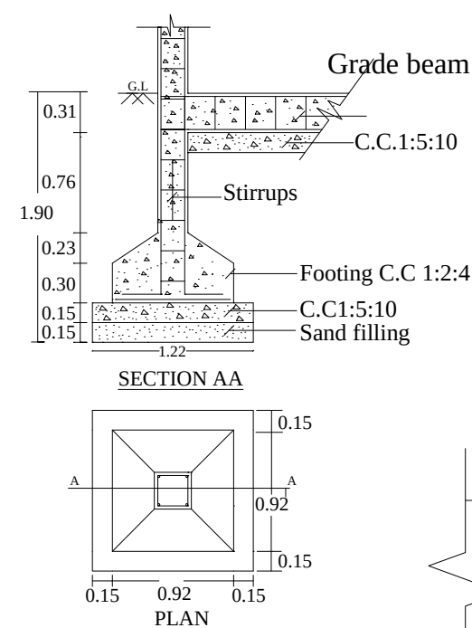
FOUNDATION DETAILS
