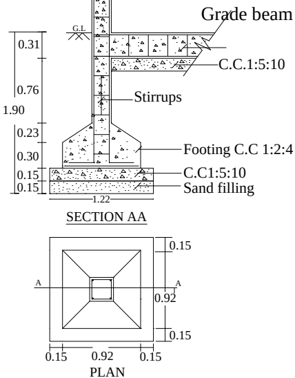
FOUNDATION DETAILS
