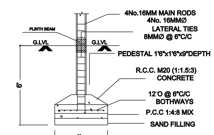
DETAIL OF R.C.C COLUMN FOOTING
