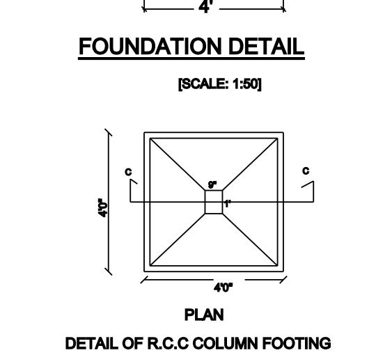
DETAIL OF R.C.C COLUMN FOOTING
