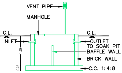
SECTION OF SEPT.TANK
