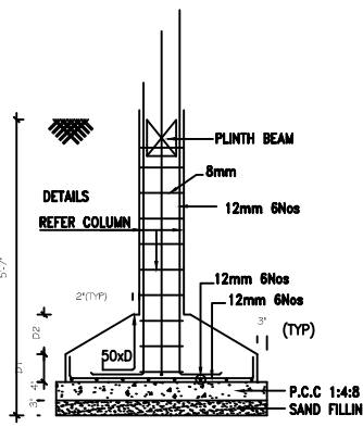
FOUNDATION DETAILS
