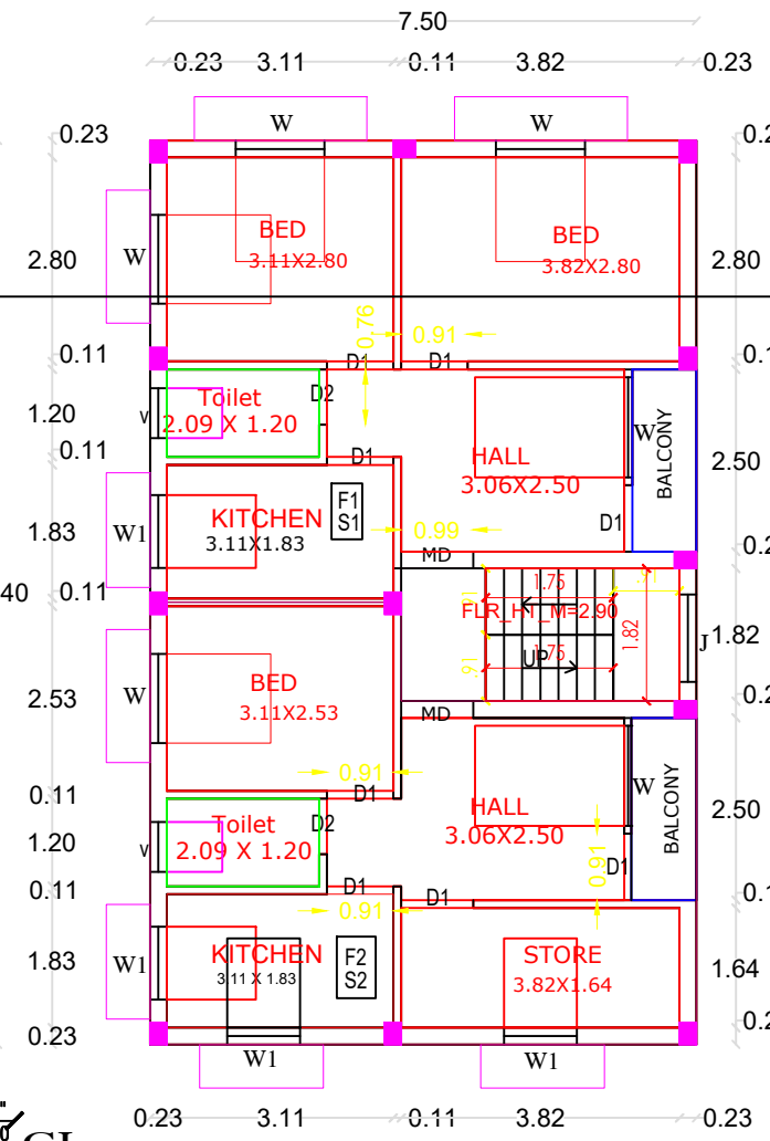
TYPICAL FLOOR PLAN=1,2 TYPICAL FLOOR PLAN (FIRST,SECOND )
