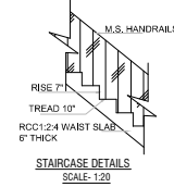
STAIRCASE DETAILS SCALE: 1/20
