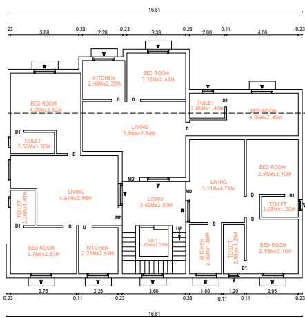
TYPICAL FIRST & SECOND FLOOR PLAN
