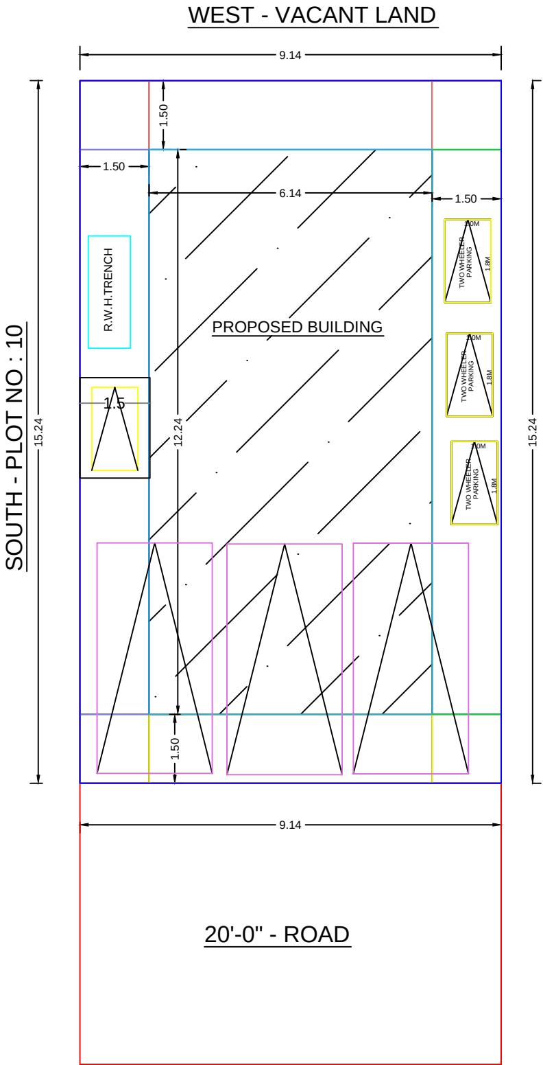
SITE PLAN
