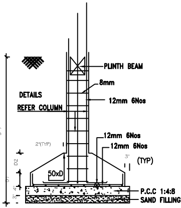
FOUNDATION DETAILS
