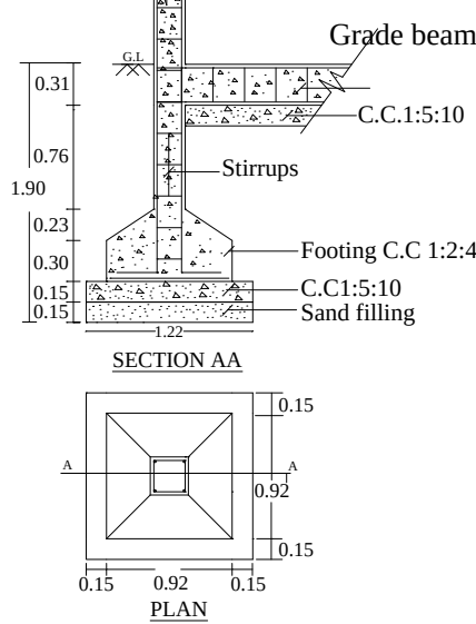
FOUNDATION DETAILS
