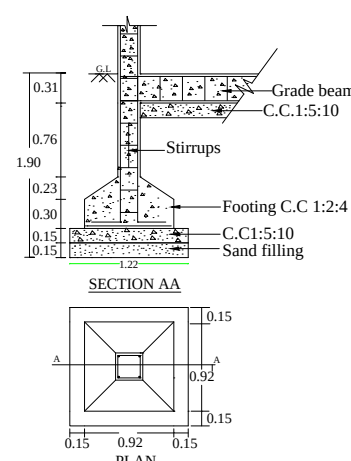
FOUNDATION DETAILS
