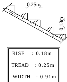
STAIRS DETAILS
