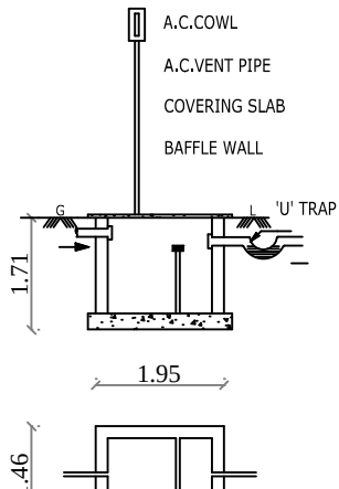
SEPTIC TANK
