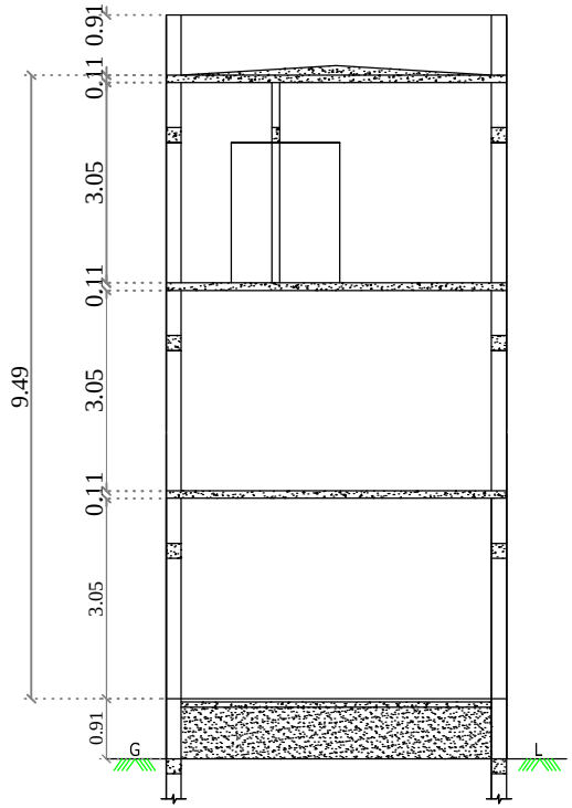
SECTION ON "SC"
