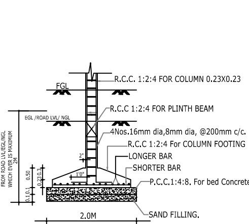
FOUNDATION DETAIL
