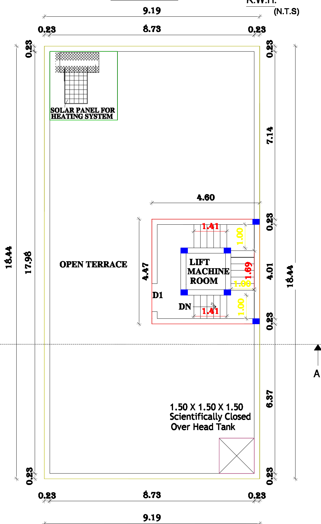
TERRACE FLOOR PLAN PROPOSED
