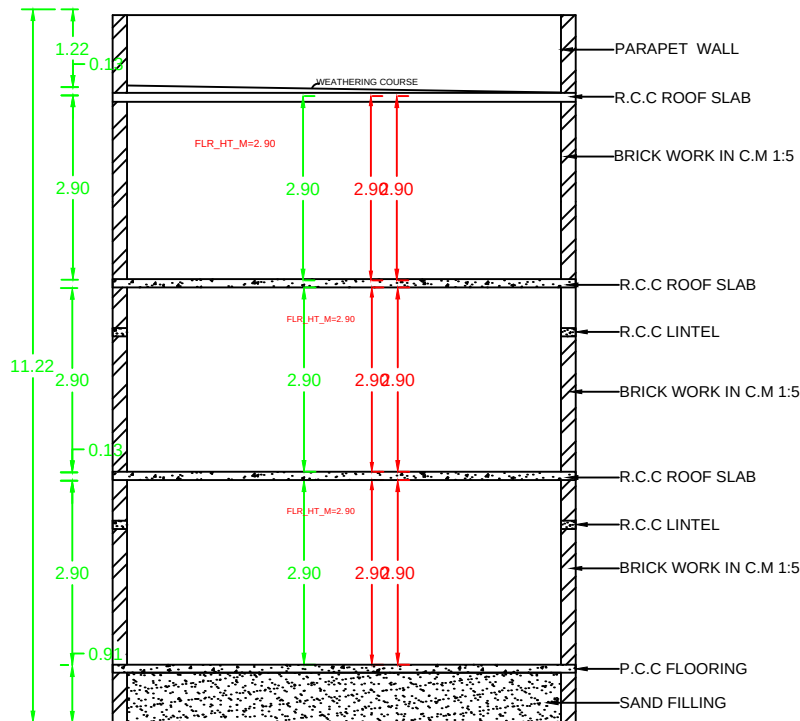
SECTION
