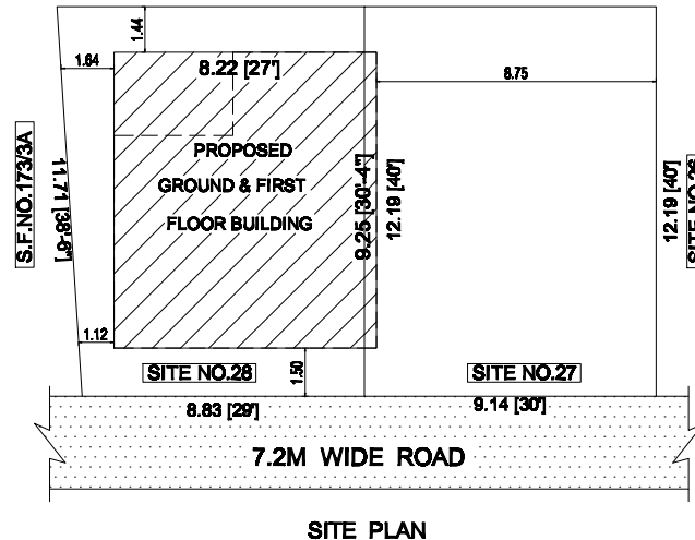
SITE PLAN
