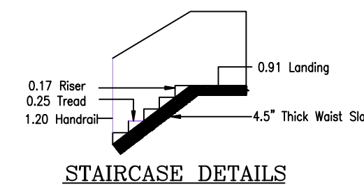
STAIRCASE DETAILS
