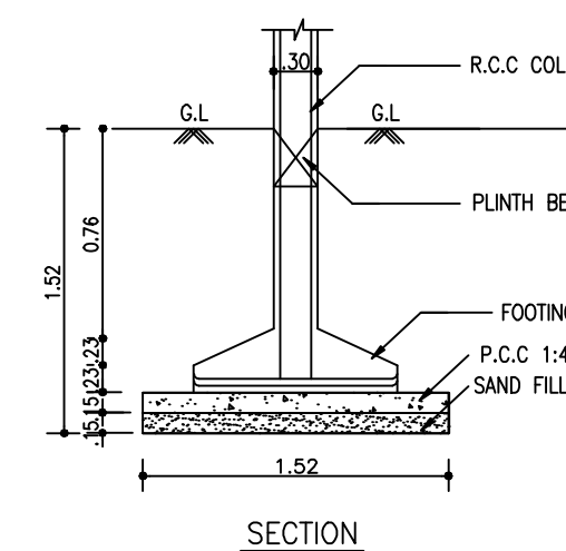
SECTION
