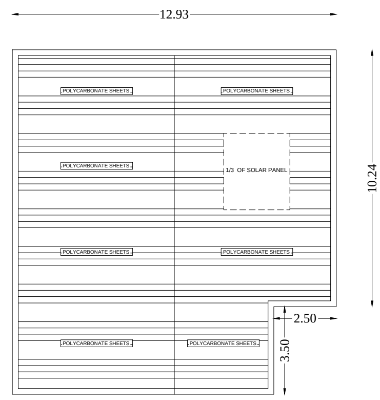
TERRACE FLOOR
