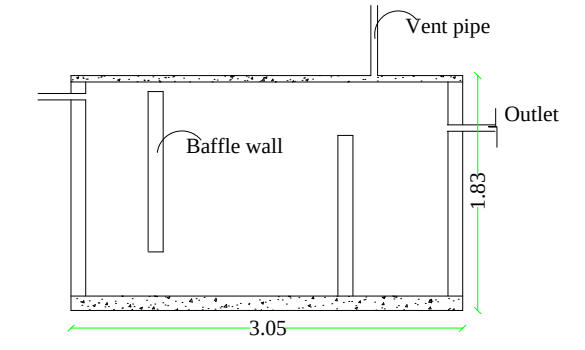
SEPTIC TANK DETAILS Size: 3.05 x 1.83 SCALE 1:100
