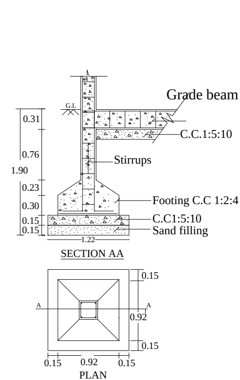
FOUNDATION DETAILS
