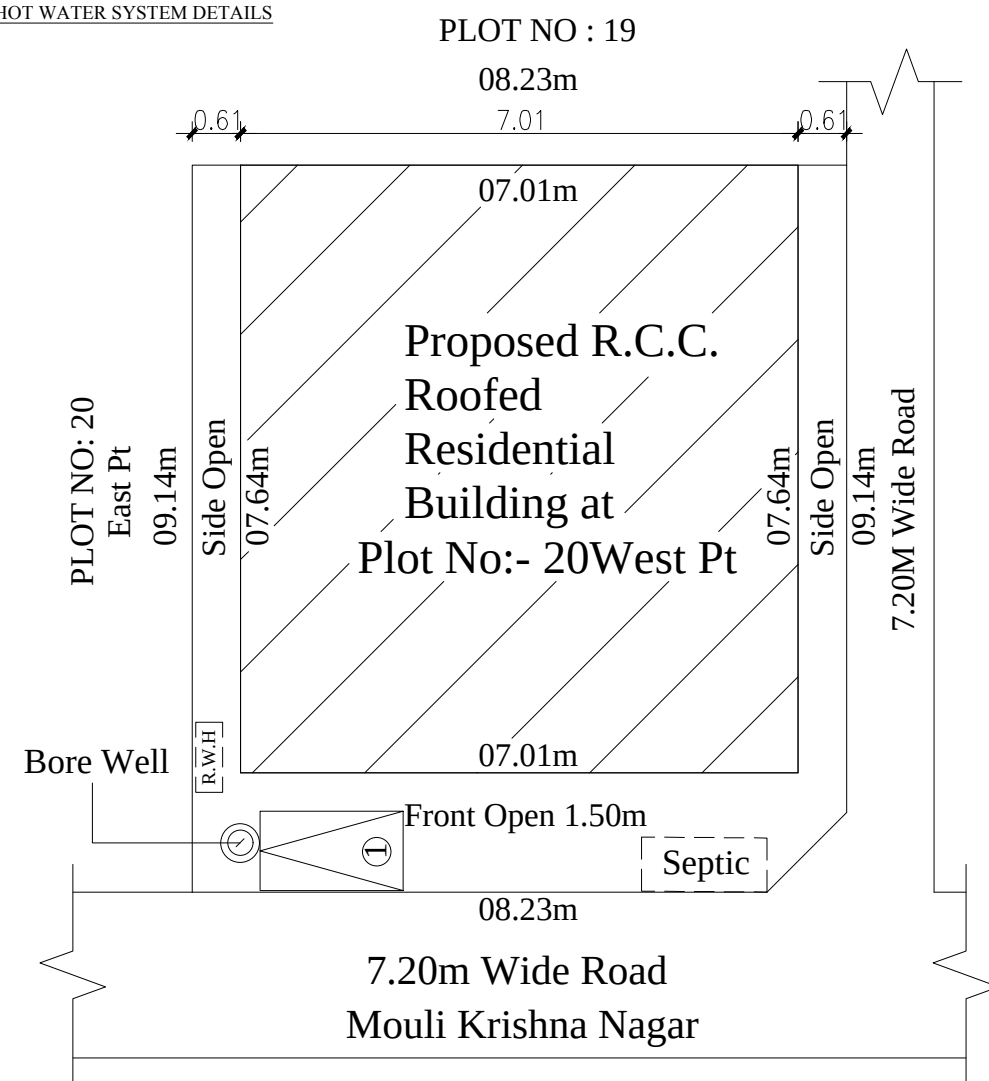
SITE PLAN
