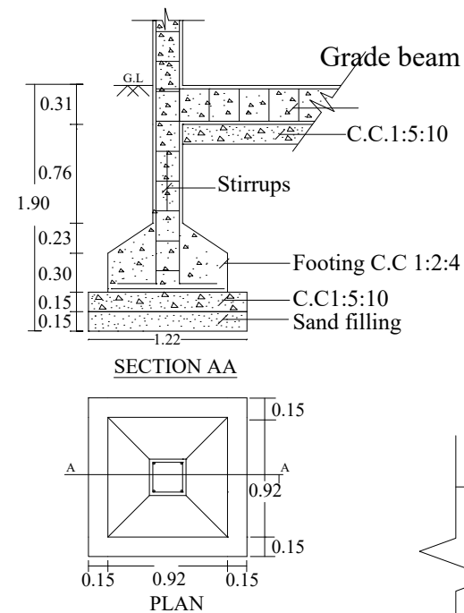
FOUNDATION DETAILS
