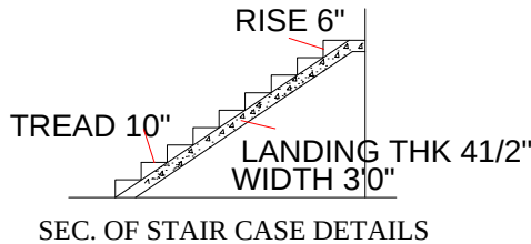
SEC. OF STAIR CASE DETAILS
