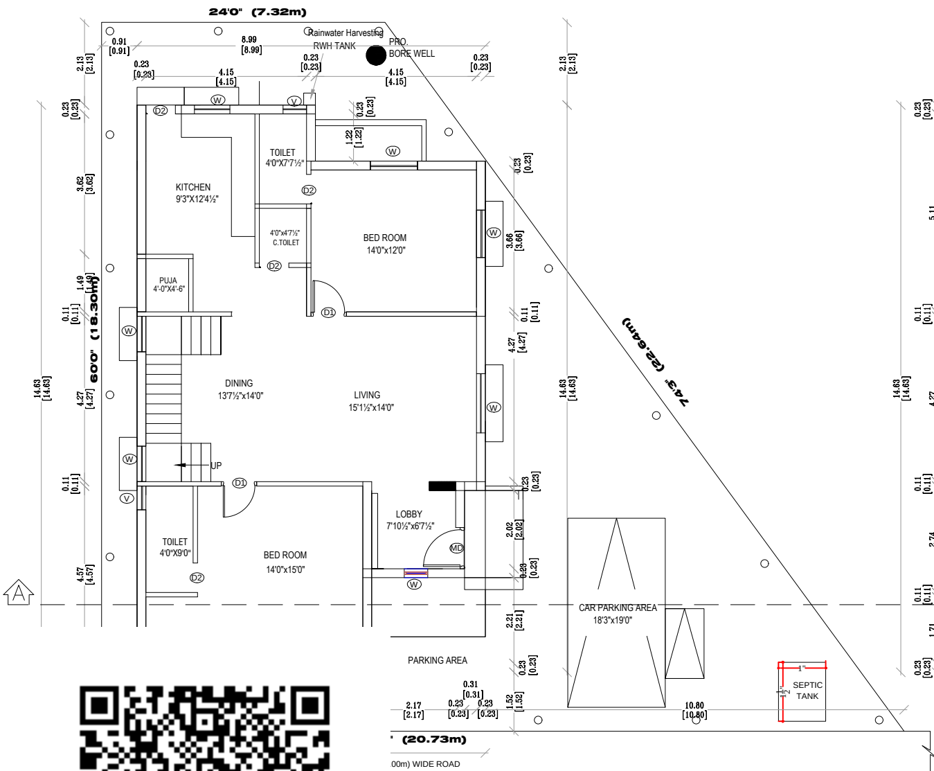
FLOOR PLAN
