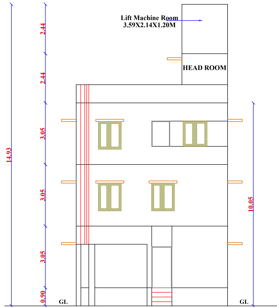
ELEVATION (PROPOSED)
