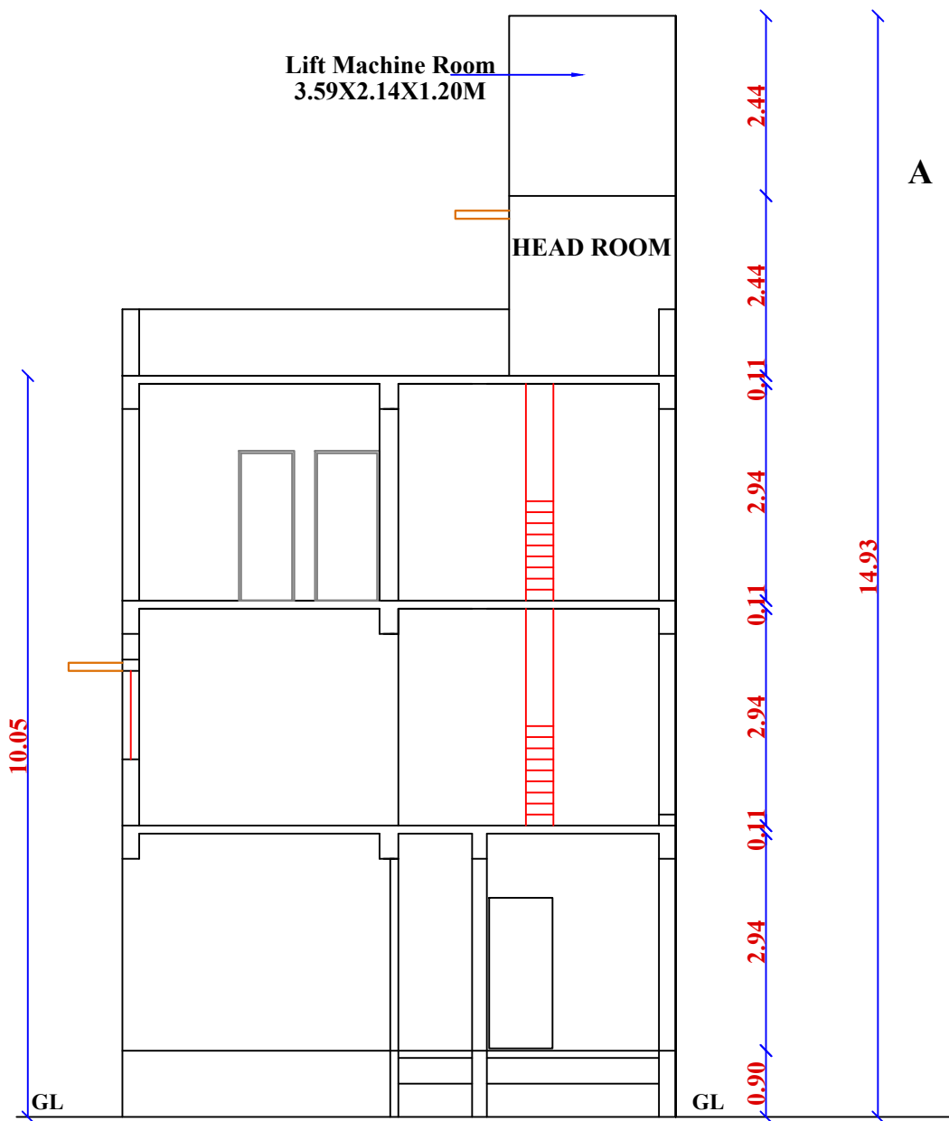
SECTION A-A (PROPOSED)
