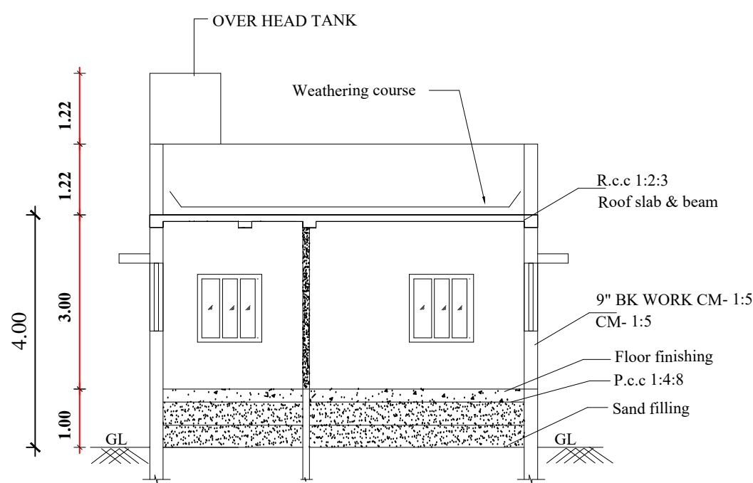
SECTION "A-B" (TO BE DEMOLISHED)
