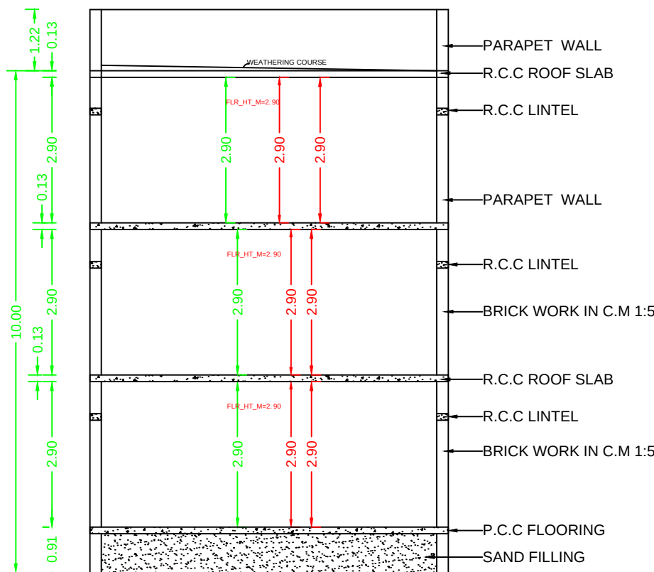
SECTION
