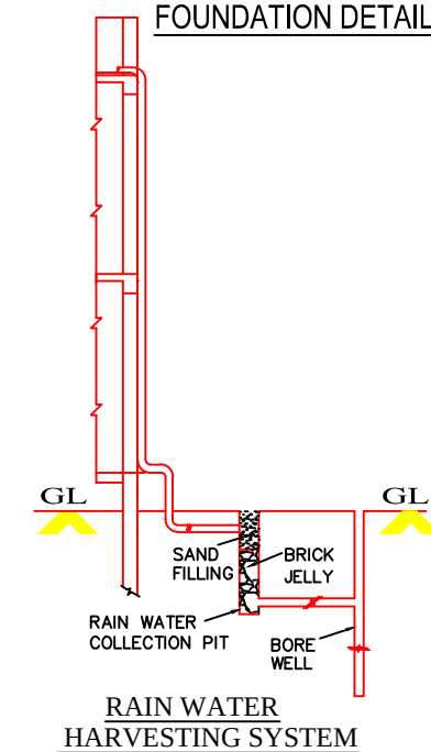
FOUNDATION DETAILS
