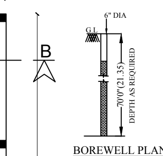
BOREWELL PLAN
