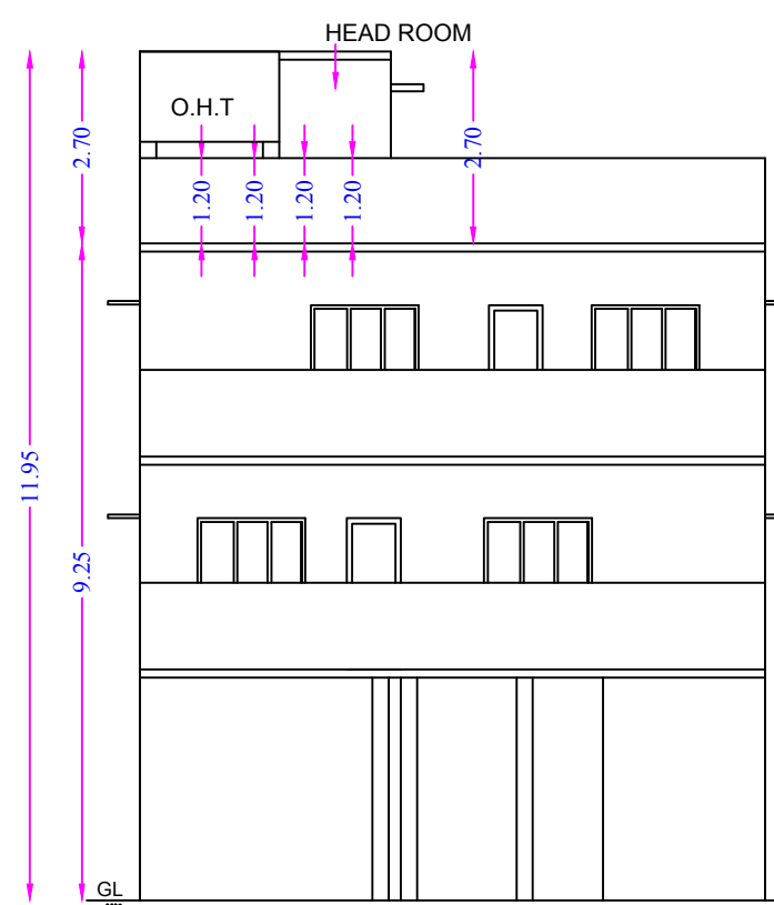
FRONT ELEVATION
