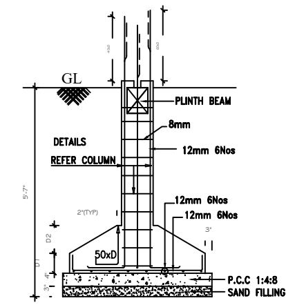
FOUNDATION DETAILS SCALE : 1:50.
