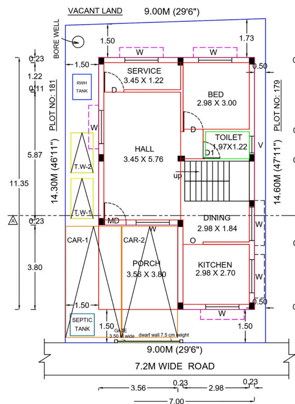
1 GROUND FLOOR PLAN
