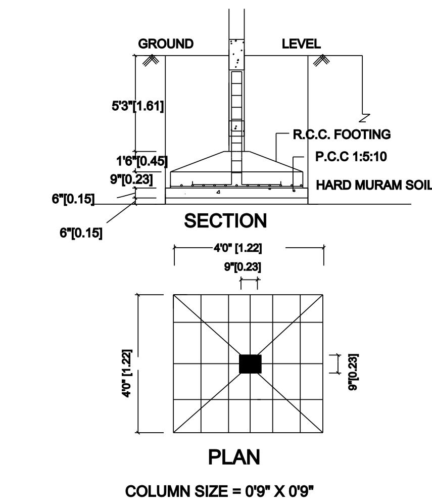
FOUNDATION DETAILS
