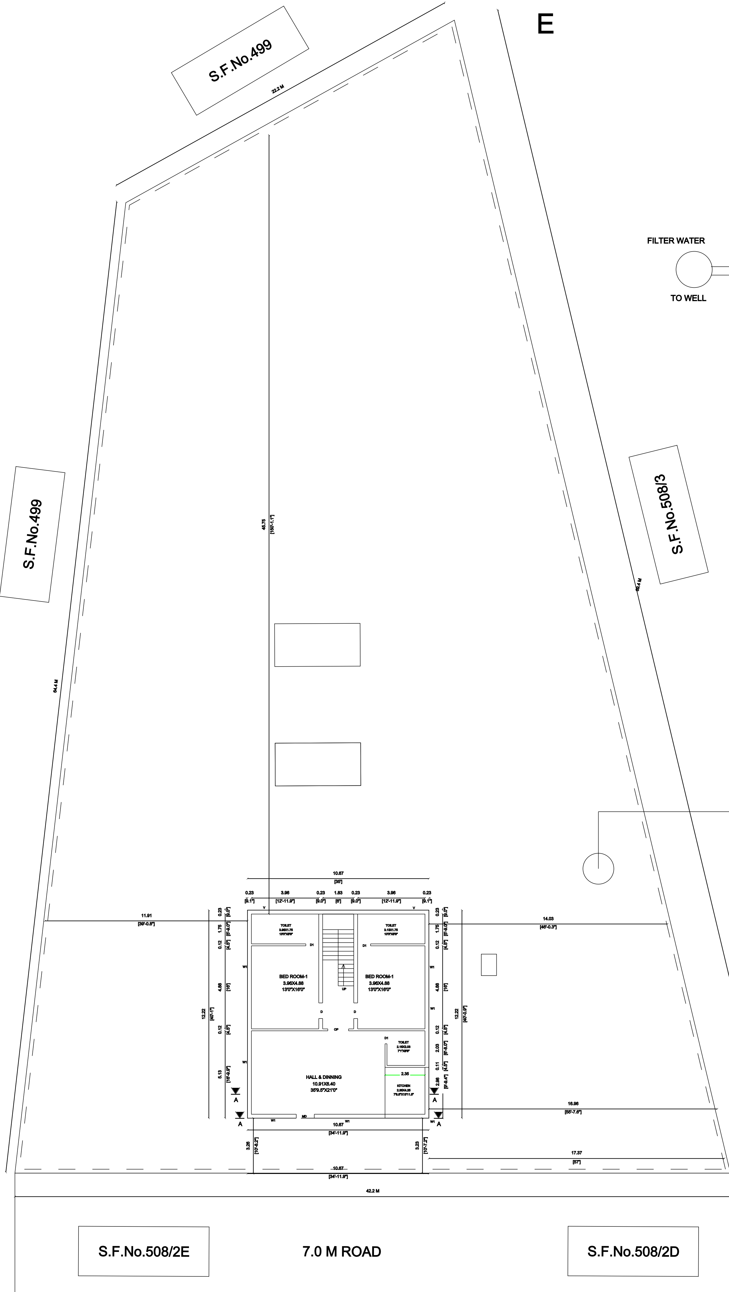
PRO. SITE CUM GROUND FLOOR PLAN
