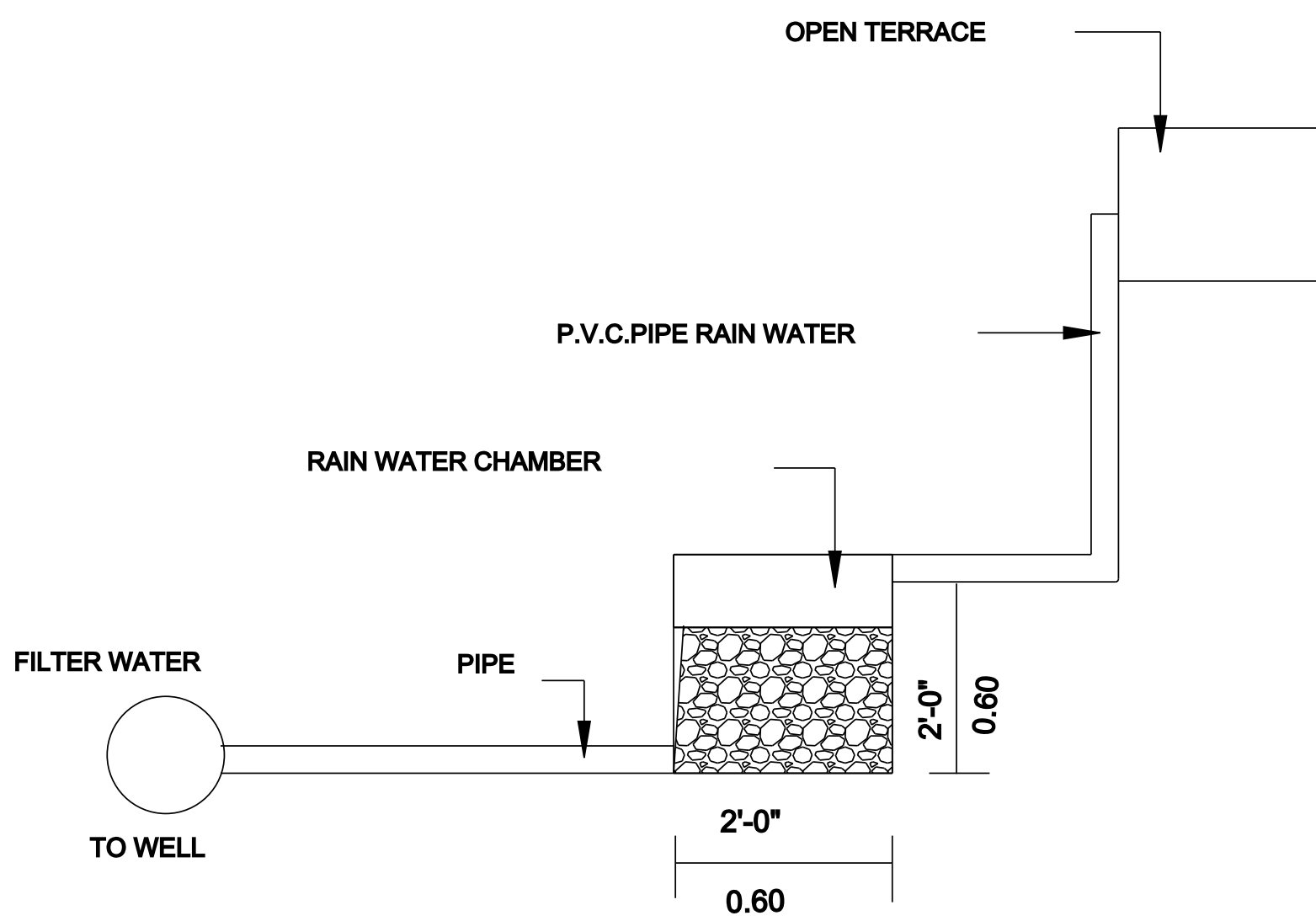
RAIN WATER HARVESTING
