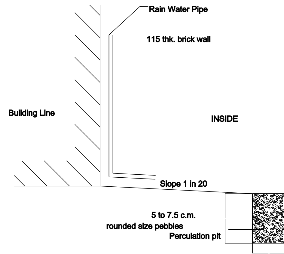
PERCOLATION PIT
