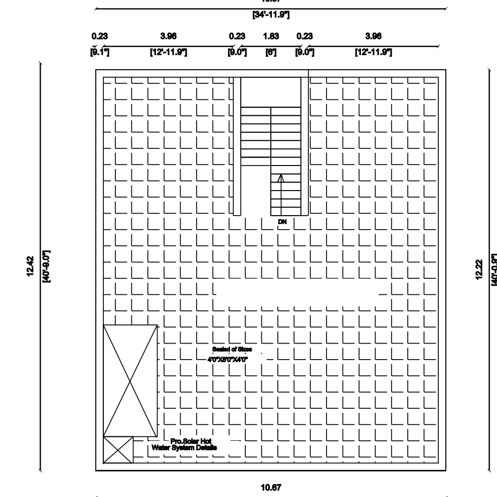
PRO. TERRACE FLOOR PLAN
