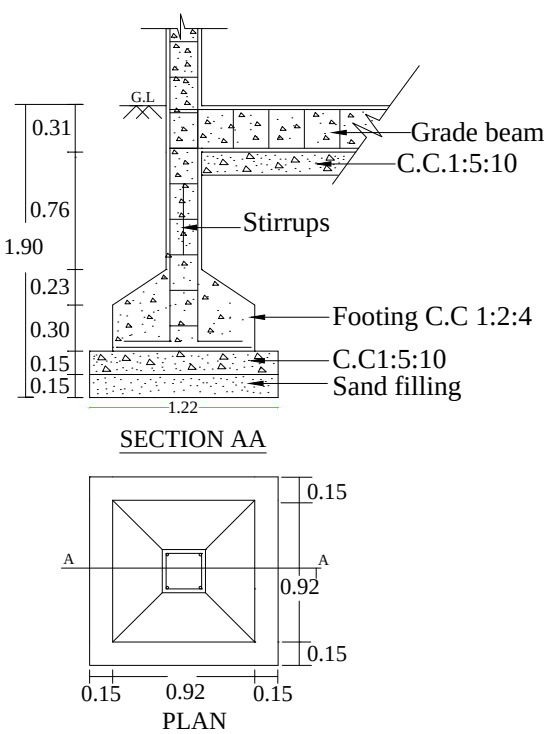
FOUNDATION DETAILS
