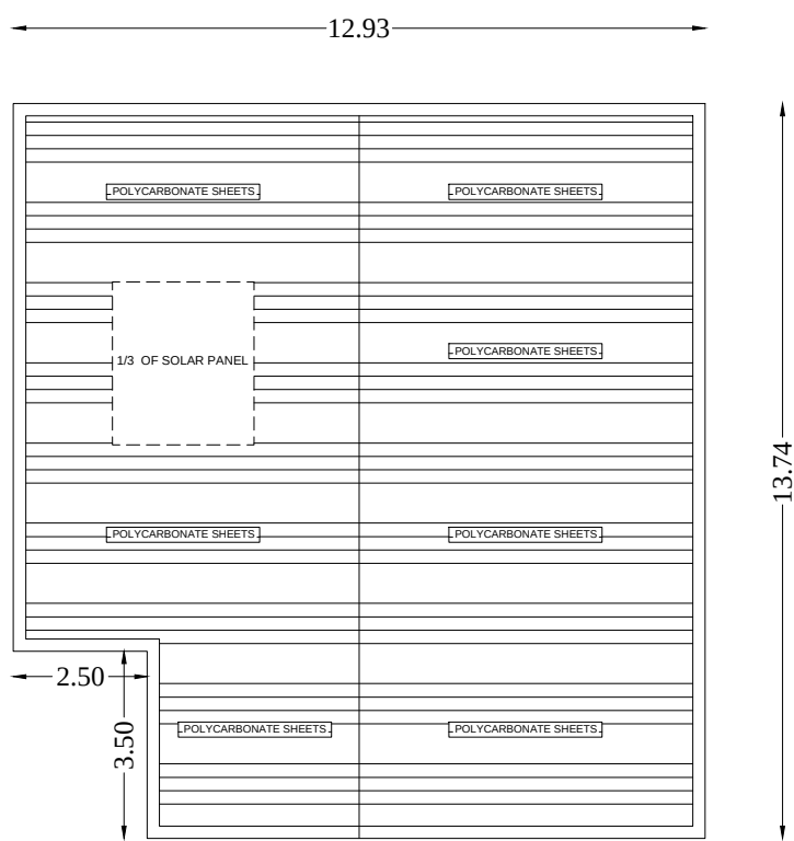
TERRACE FLOOR
