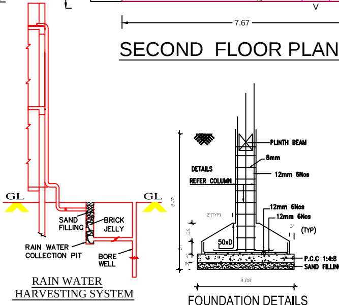
FOUNDATION DETAILS
