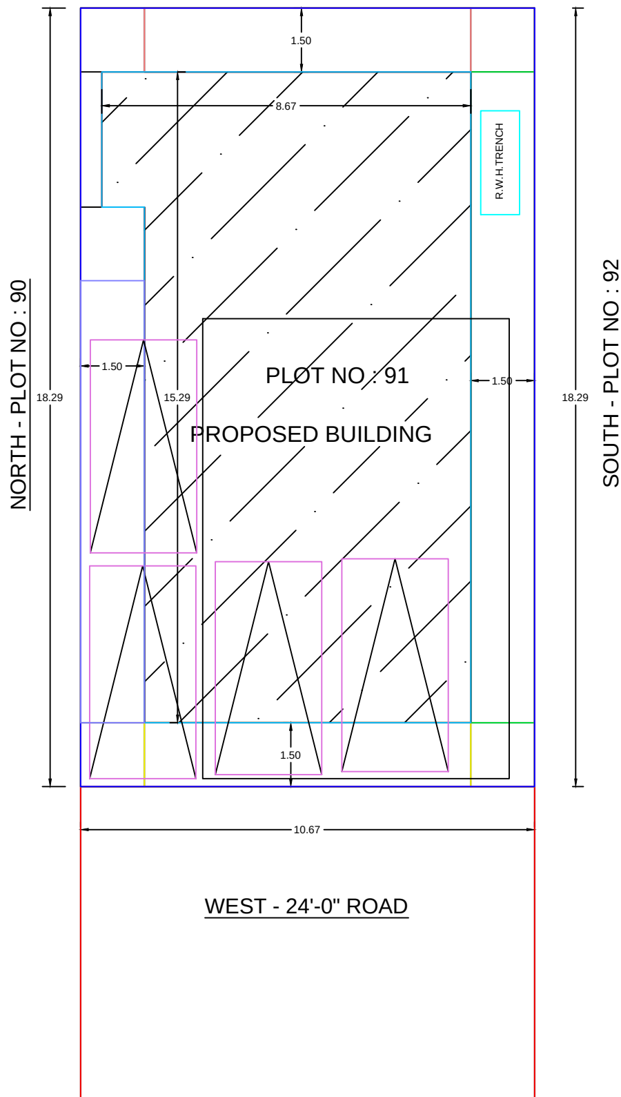
SITE PLAN
