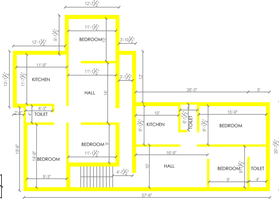
FIRST FLOOR PLAN ( TO BE DEMOLISHED )
