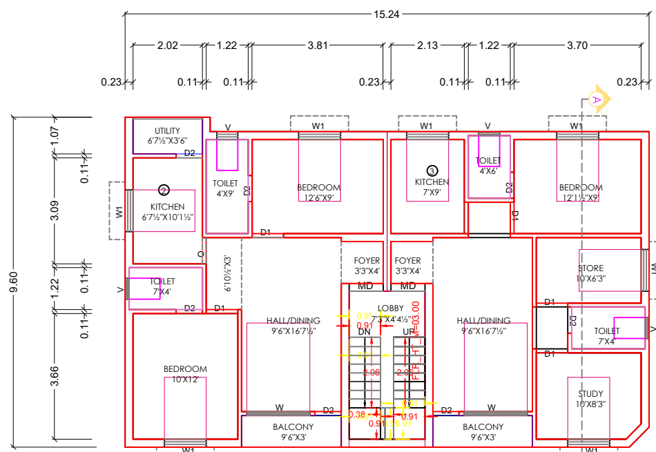
GROUND FLOOR PLAN ( TO BE DEMOLISHED )
