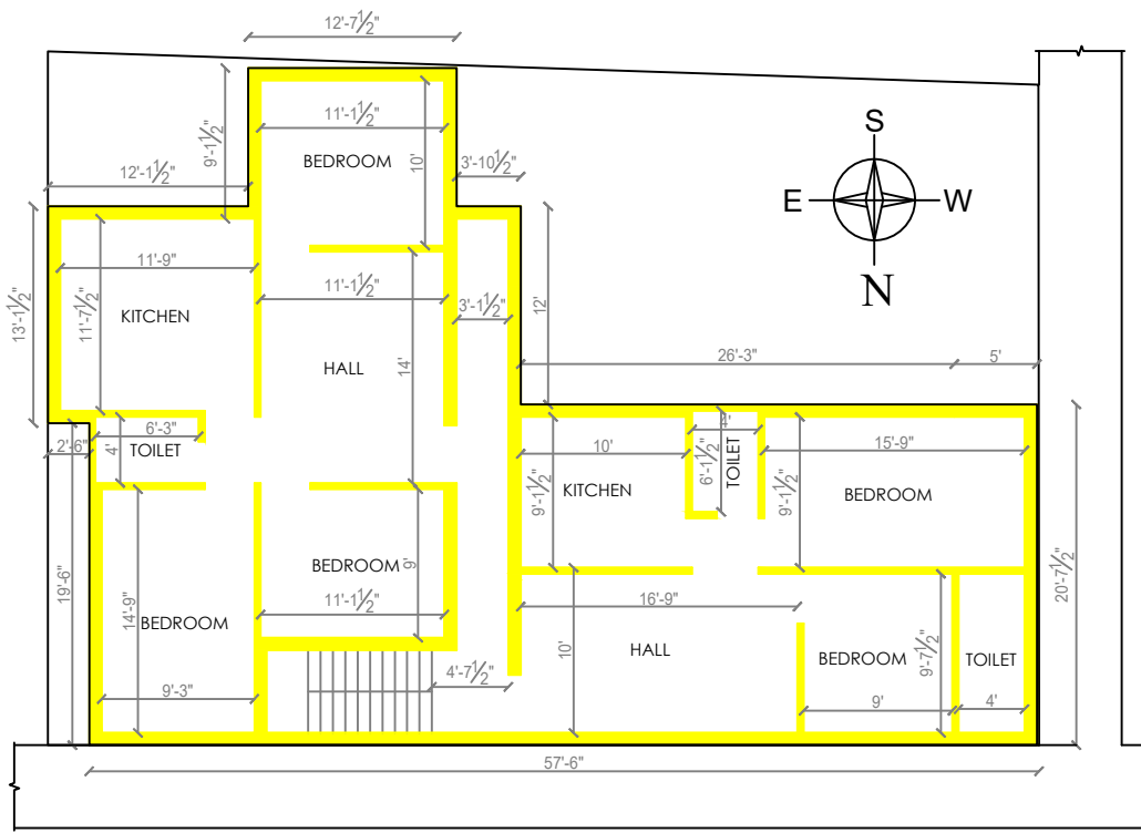
GROUND FLOOR PLAN ( TO BE DEMOLISHED )
