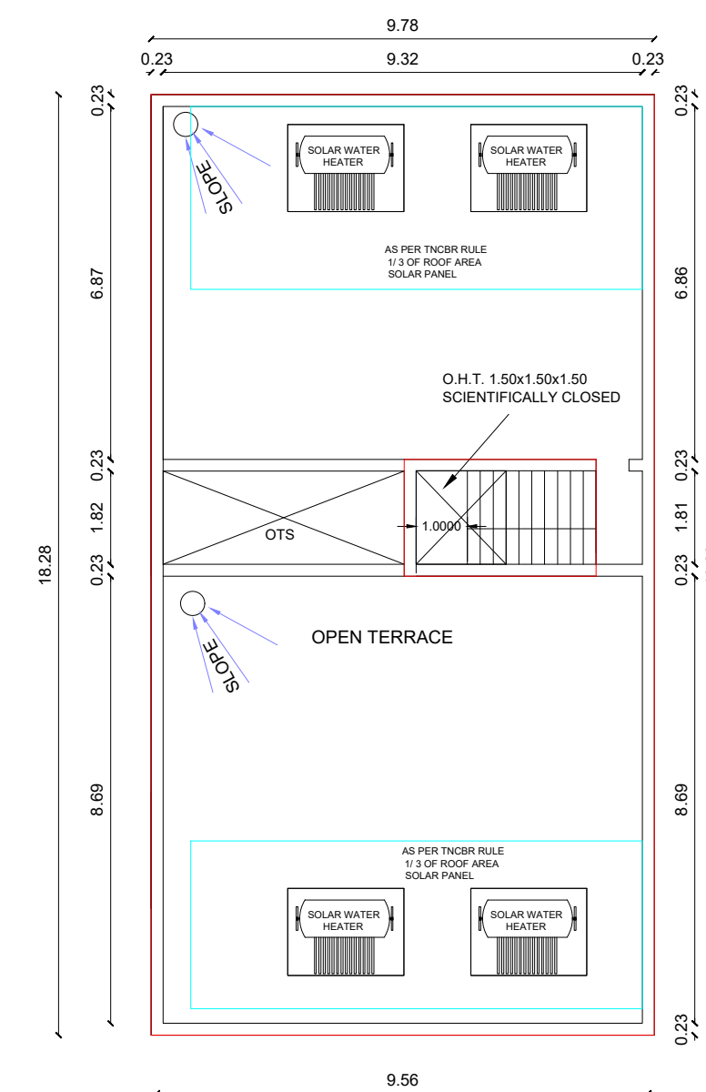
TERRACE FLOOR PLAN (PROPOSED)
