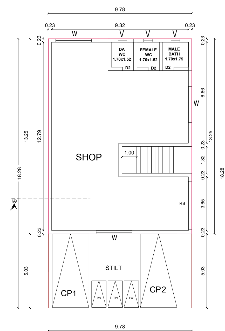
GROUND FLOOR PLAN (PROPOSED)
