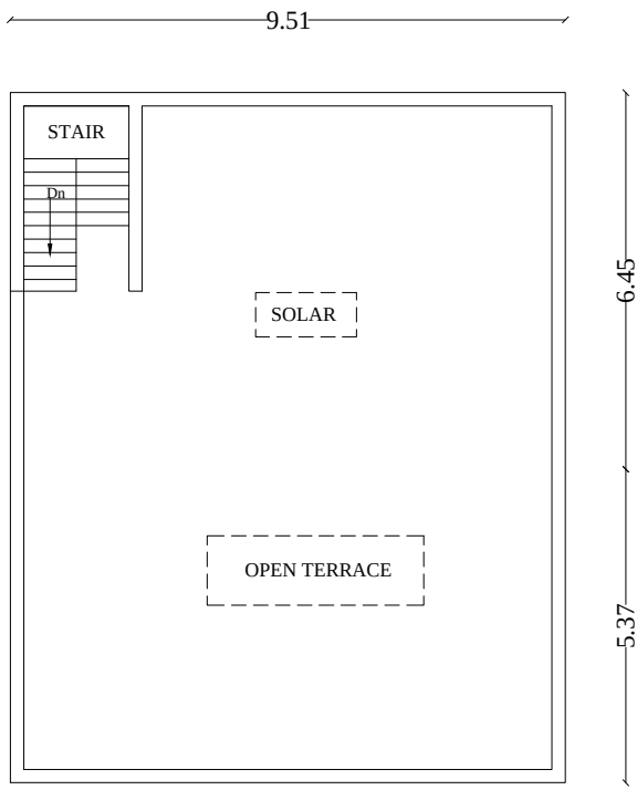
TERRACE FLOOR
