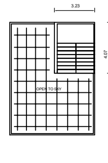
TERRACED FLOOR PLAN
