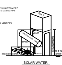
HEATING SYSTEM
