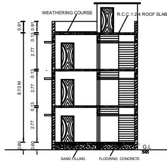
SECTION ON " MS "
