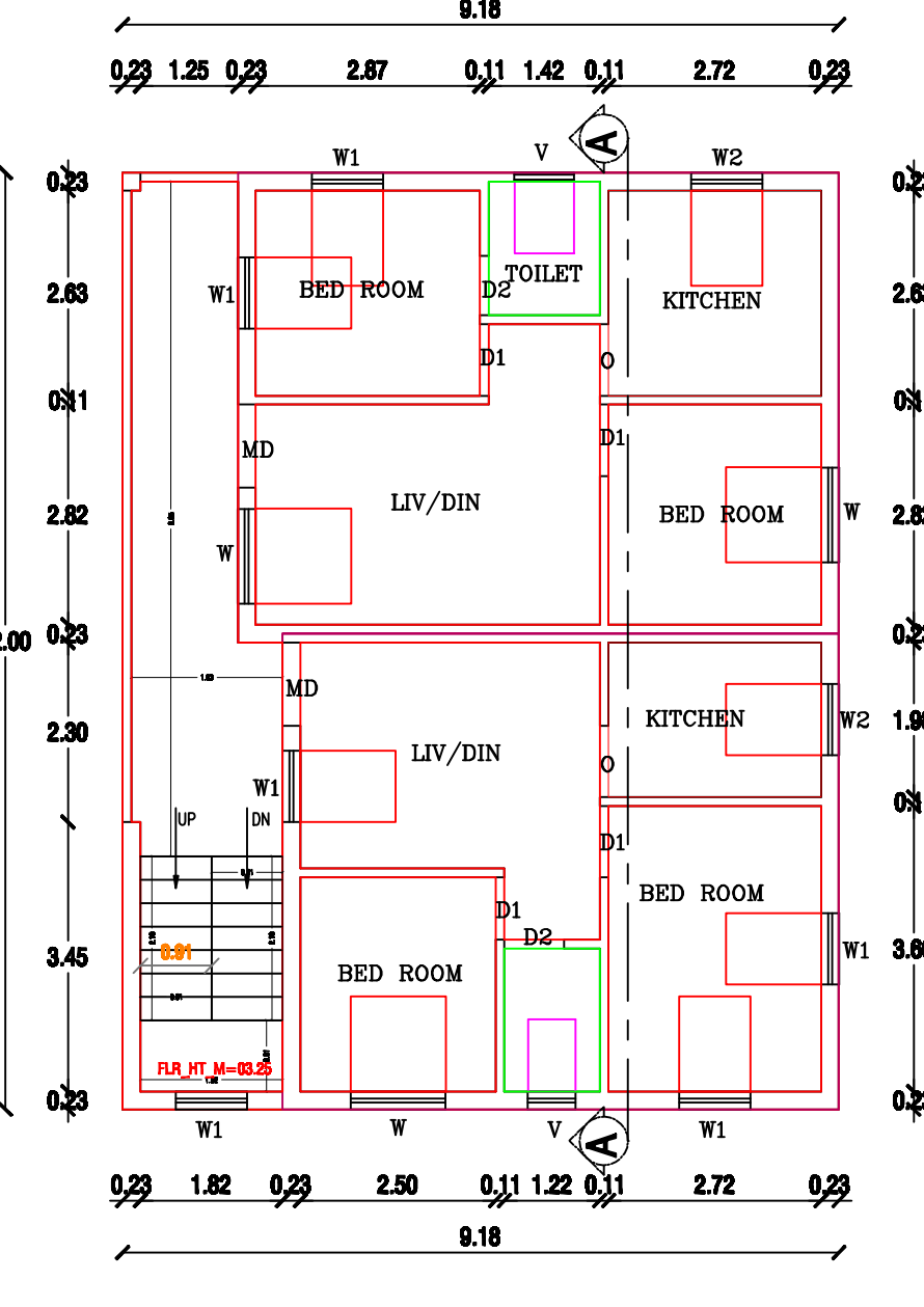
FIRST FLOOR PLAN (PROPOSED)
