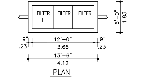
SEPTIC TANK DETAIL
