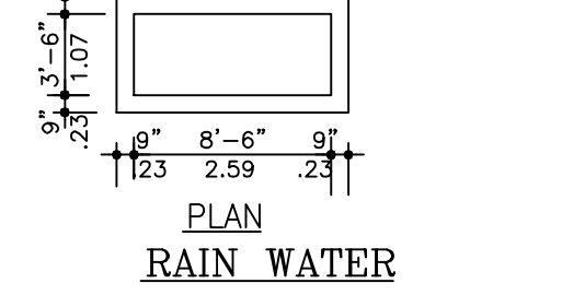
RAIN WATER HARVESTING TANK DETAIL
