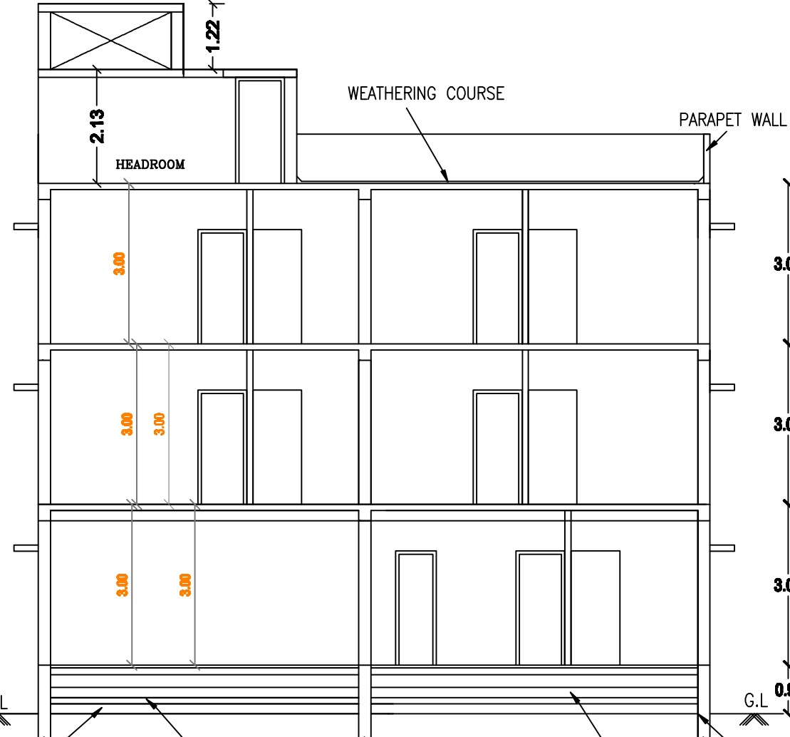
SECTION 'A-A'
