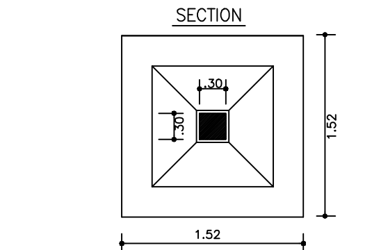
FOUNDATION DETAIL
