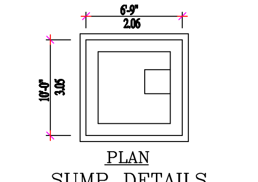
SUMP DETAILS (SCIENTIFICALLY CLOSED)
