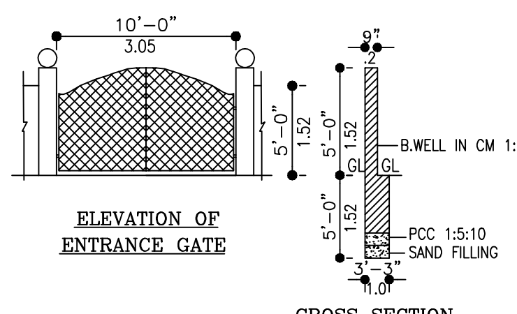
ELEVATION OF ENTRANCE GATE
