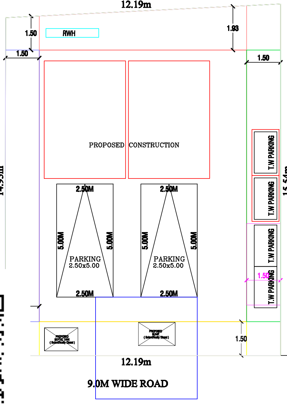
SITE PLAN (PROPOSED)
