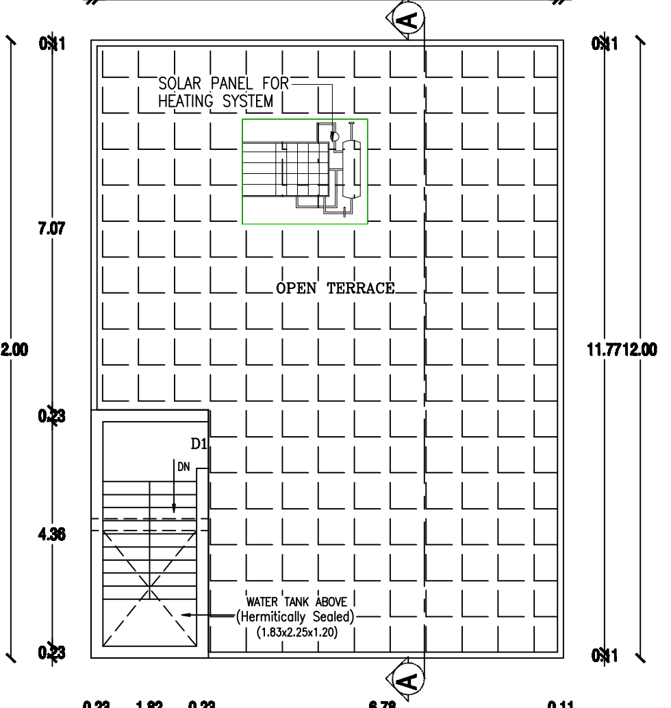
TERRACE FLOOR PLAN (PROPOSED)
