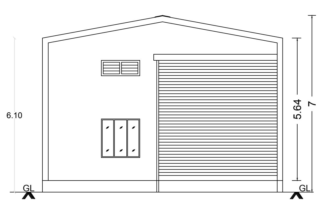
FRONT ELEVATION
