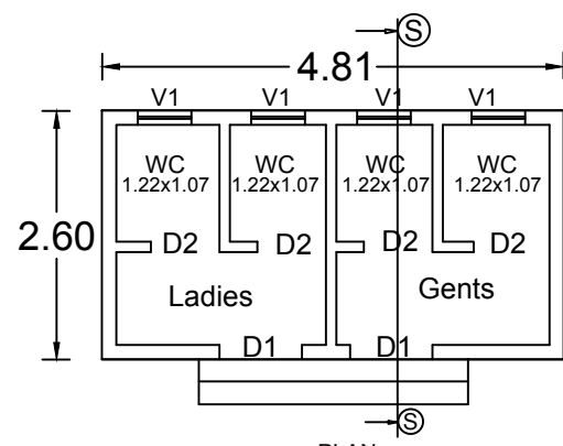
TOILET DETAILS
