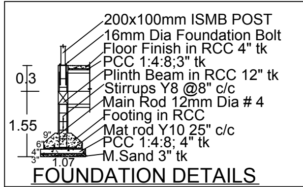
FOUNDATION DETAILS
