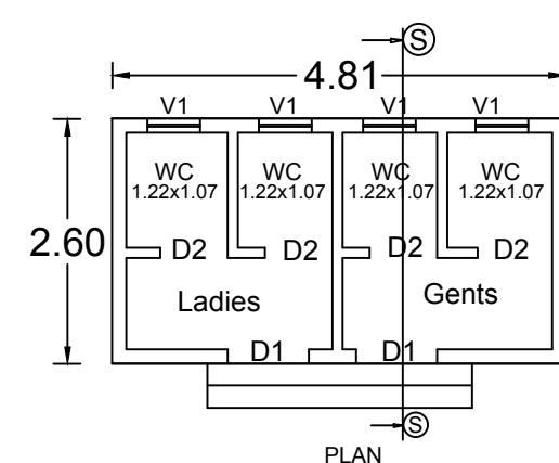
TOILET DETAILS
