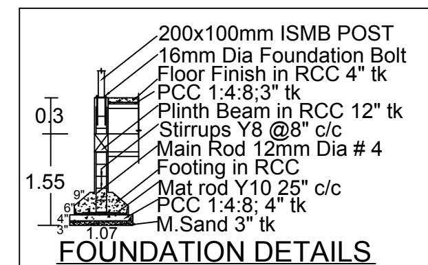
FOUNDATION DETAILS
