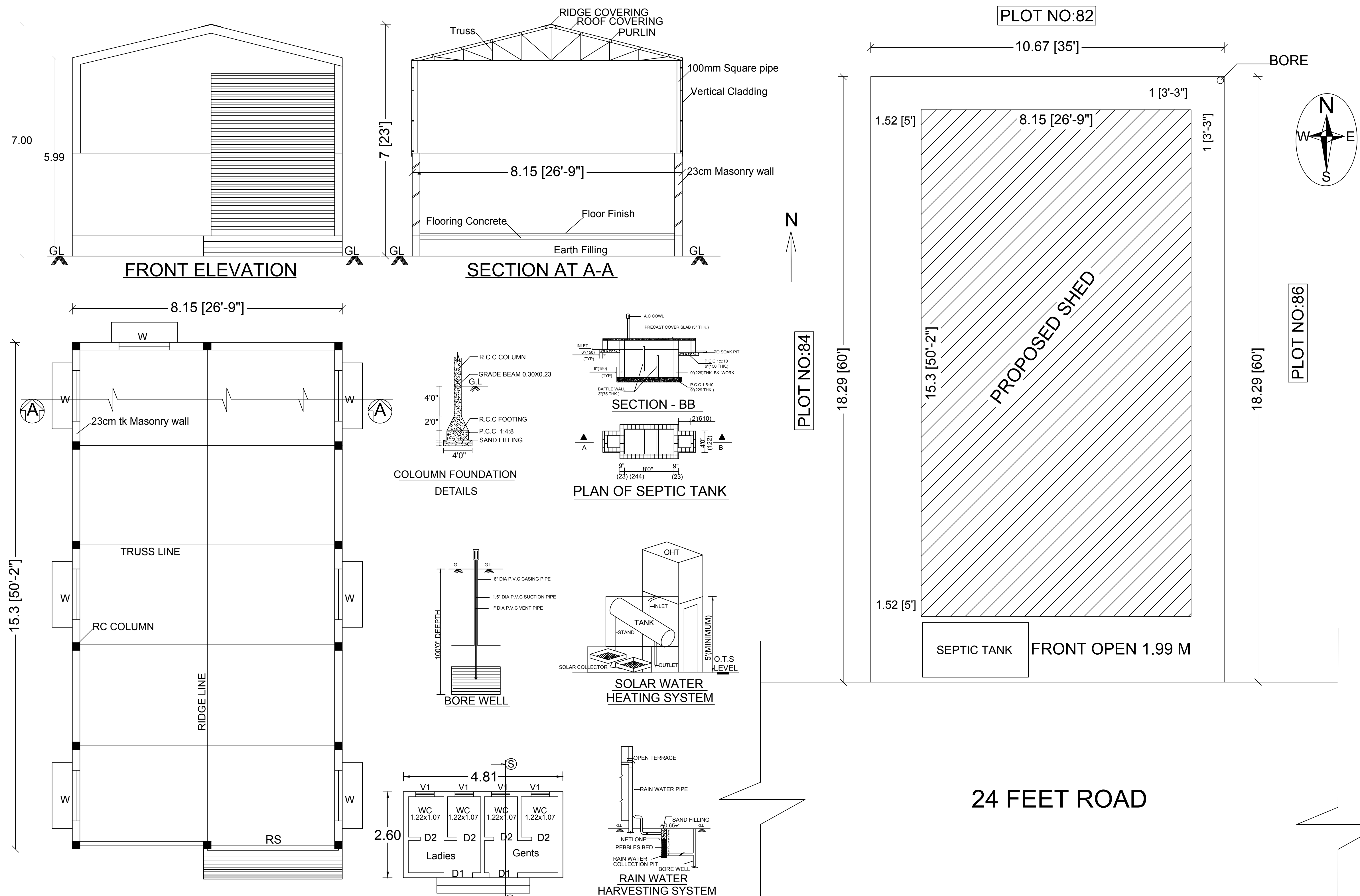
OSD SHED PLAN SCALE 1:100
