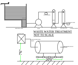
SOLOR HOT WATER SYSTEM DETAILS
