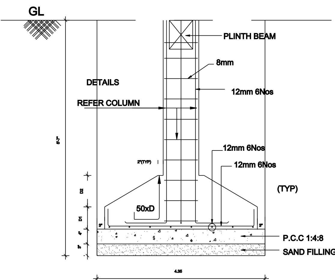
FOUNDATION DETAILS
