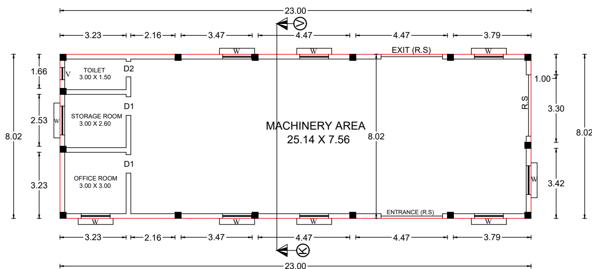
PROPOSED GROUND FLOOR
