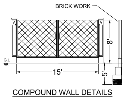
COMPOUND WALL DETAILS
