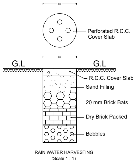
RAIN WATER HARVESTING (Scale 1 : 1)
