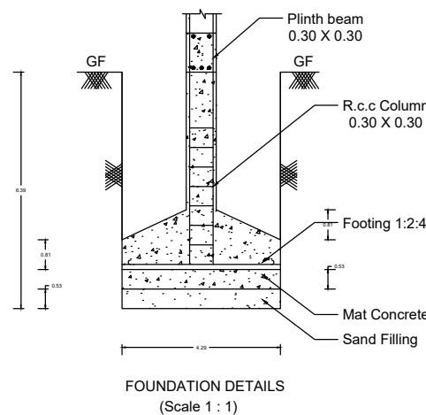
FOUNDATION DETAILS (Scale 1 : 1)
