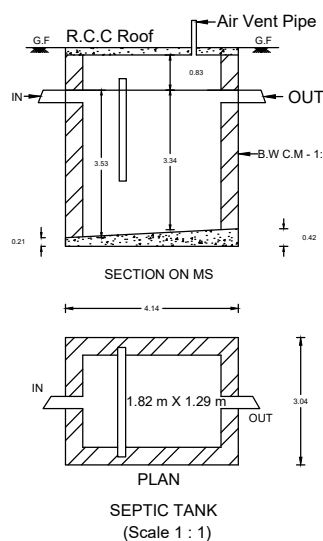
SEPTIC TANK (Scale 1 : 1)
