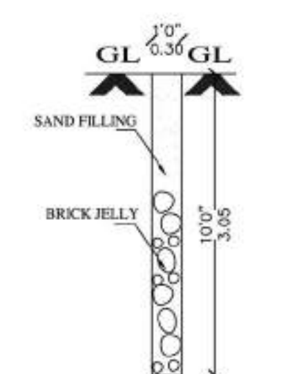
PERCULATION PIT
