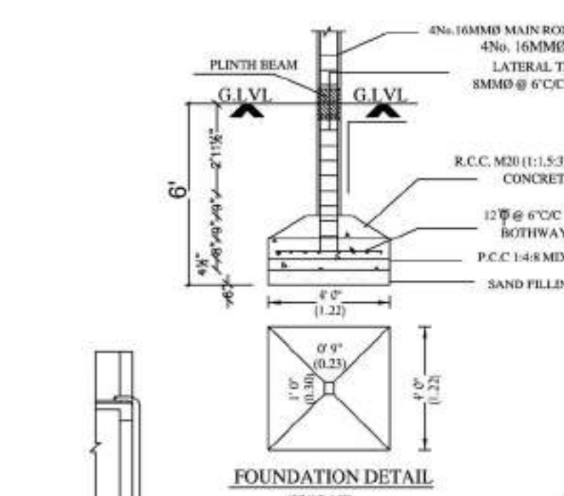
FOUNDATION DETAIL
