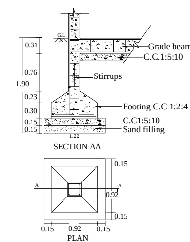
FOUNDATION DETAILS
