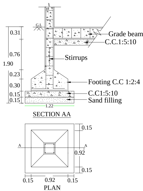
FOUNDATION DETAILS
