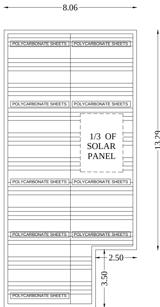
TERRACE FLOOR
