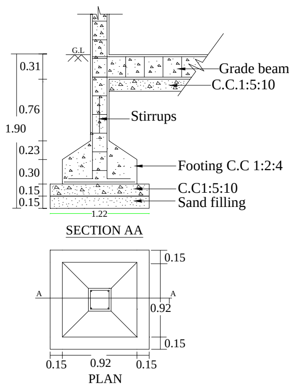
FOUNDATION DETAILS
