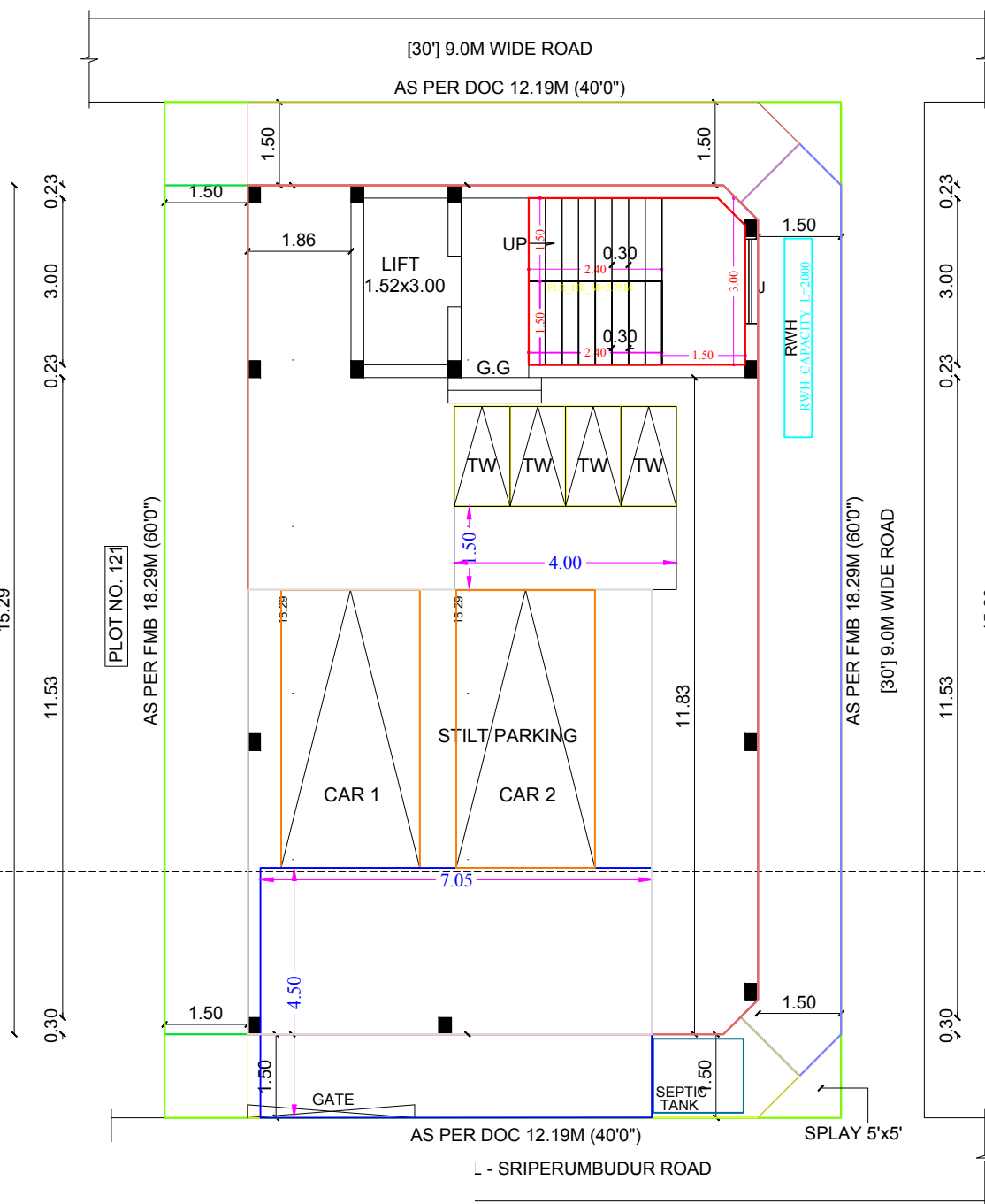
LT FLOOR PLAN
