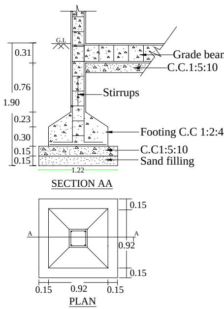
FOUNDATION DETAILS
