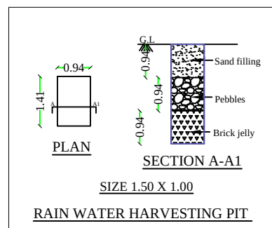
RAIN WATER HARVESTING PIT
