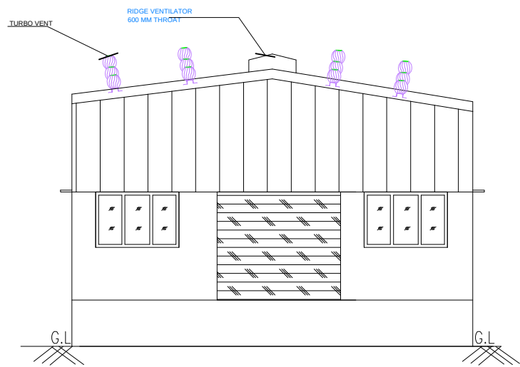
FRONT ELEVATION
