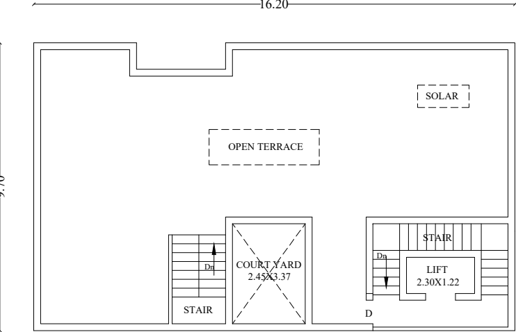
TEERACE FLOOR
