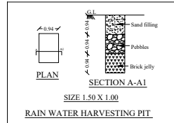
RAIN WATER HARVESTING PIT
