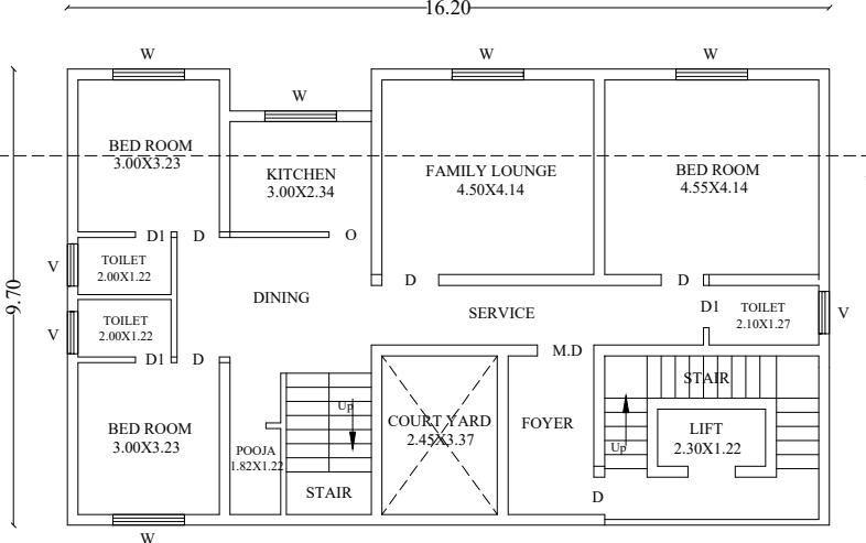
THIRD FLOOR
