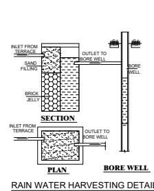
RAIN WATER HARVESTING DETAIL
