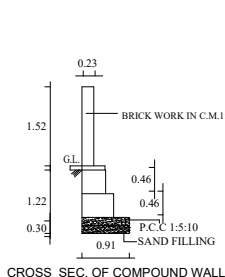
CROSS SEC. OF COMPOUND WALL
