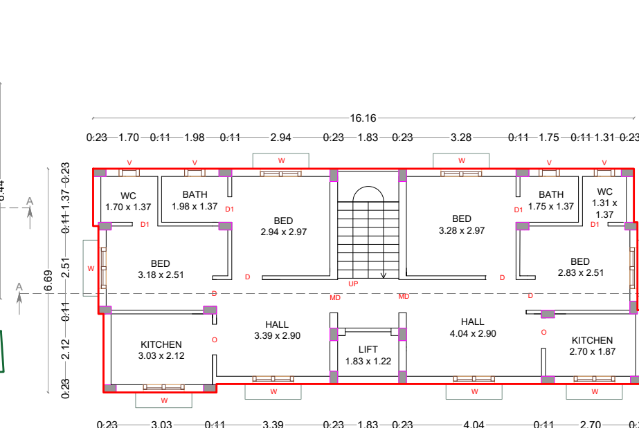
PROPOSED TYPICAL 1, 2 & 3 FLOOR PLAN
