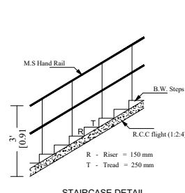
STAIRCASE DETAIL
