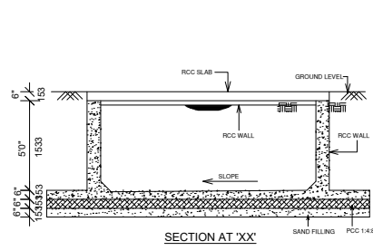
SECTION AT 'XX'
