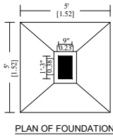
PLAN OF FOUNDATION
