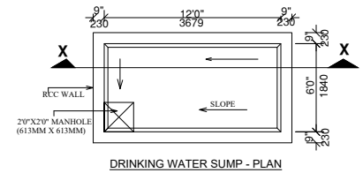
DRINKING WATER SUMP - PLAN
