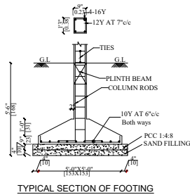
TYPICAL SECTION OF FOOTING
