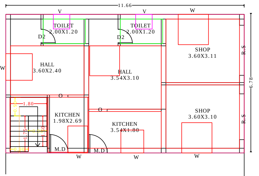
ND FLOOR PLAN
