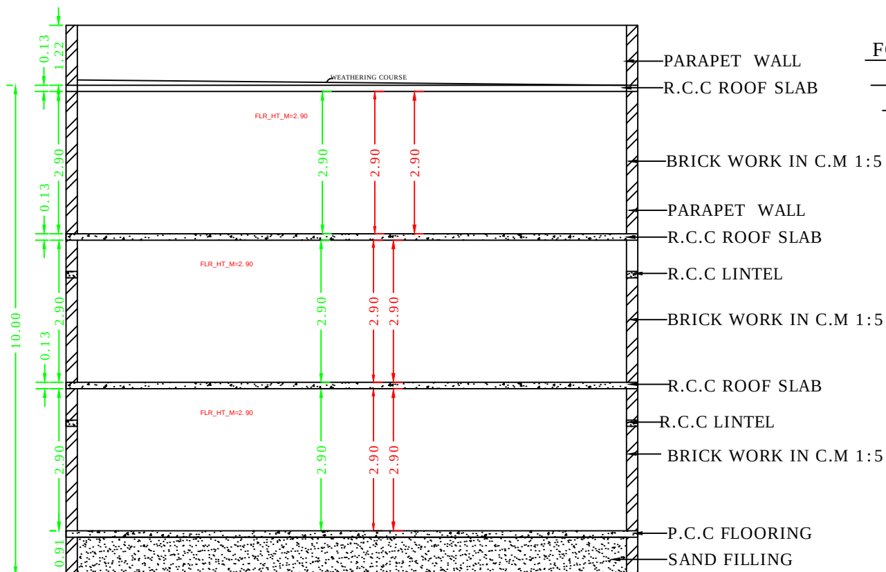
SECTION
