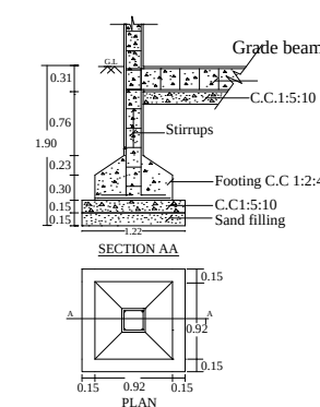
FOUNDATION DETAILS
