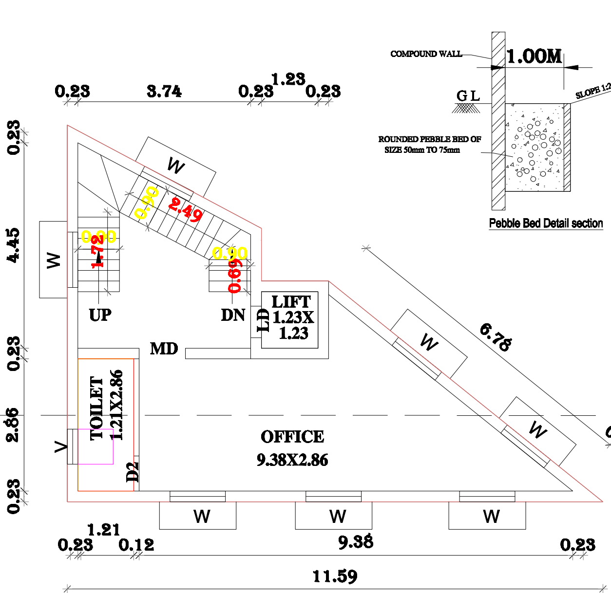
TYPICAL- I, II & III FLOOR PLAN
