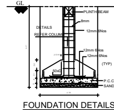
FOUNDATION DETAILS
