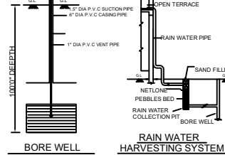
BORE WELL
